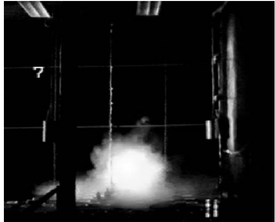
Air flow from a conventional floor-mounted swirl diffuser: minor penetration depth = risk of cold air accumulation
